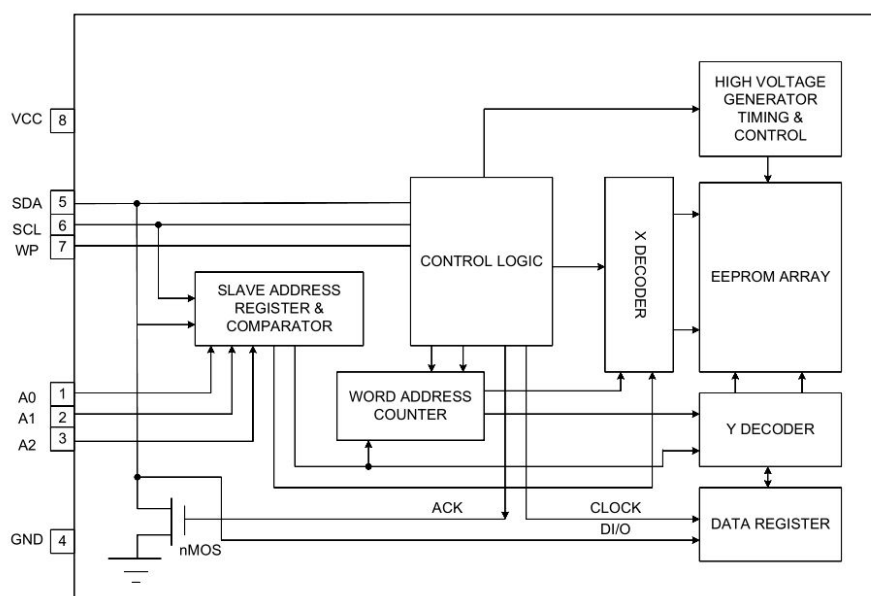
Figure 3.1 Block Diagram
