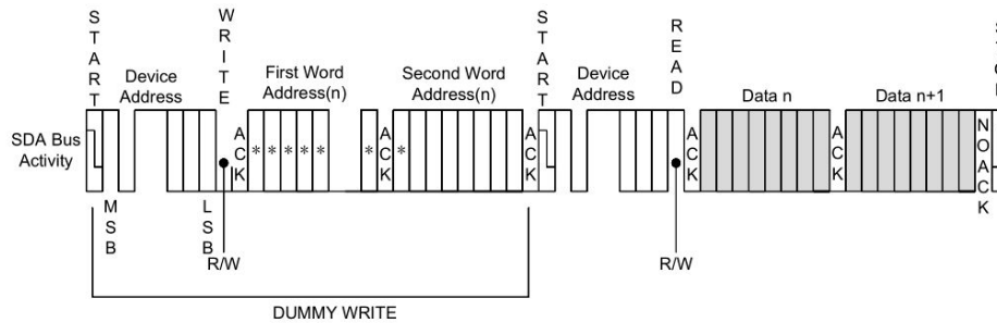
Figure 10.5 Read Security Sector
