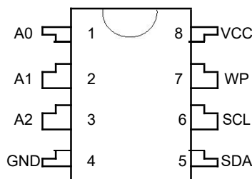
Figure 5.3 8-Pin PDIP
