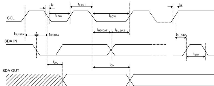
Figure 11.1 Bus Timing
