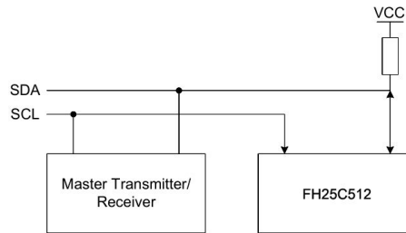
Figure 7.1 Typical System Bus Configuration
