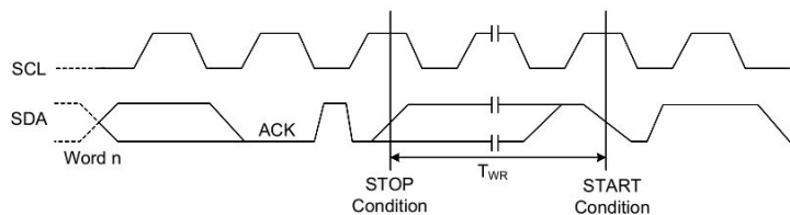
Figure 11.2 Write Cycle Timing
