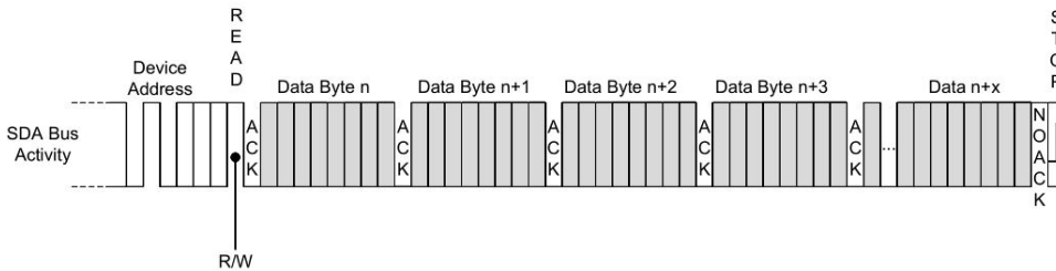
Figure 10.3 Sequential Read
