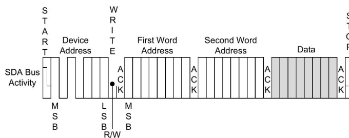
Figure 9.1 Byte Write
