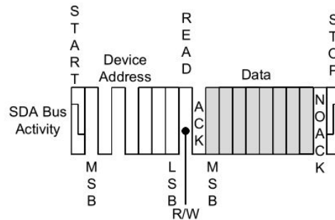
Figure 10.1 Current Address Read
