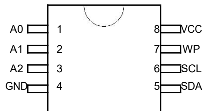
Figure 5.1 8-Pin SOIC and TSSOP
