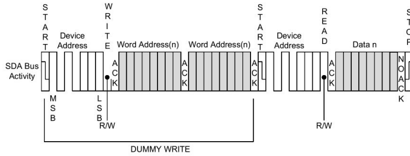
Figure 10.2 Random Read
