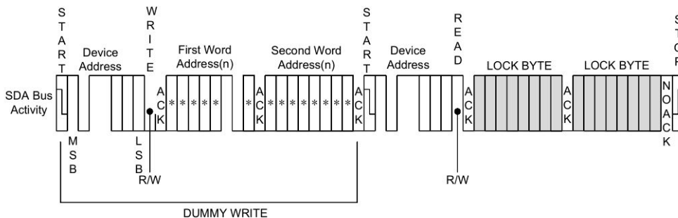
Figure 10.6 Read Lock Status
