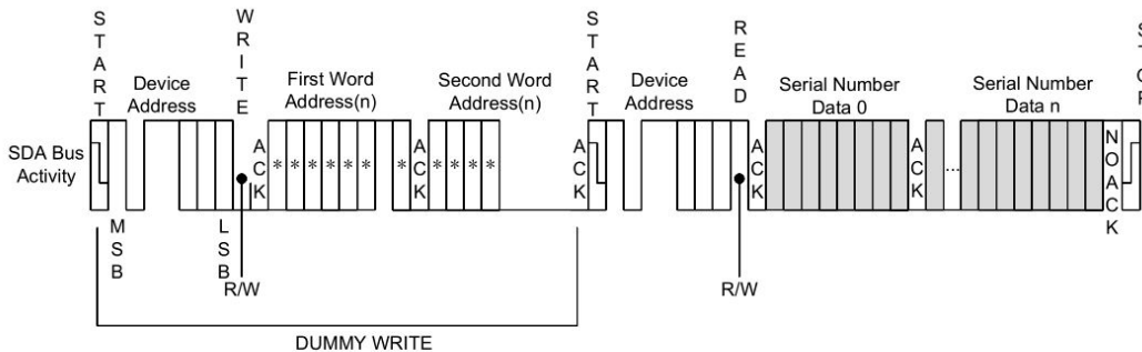
Figure 10.4 Read Unique ID
