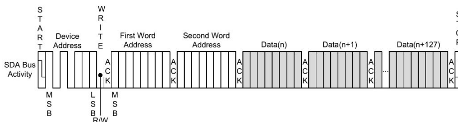
Figure 9.2 Page Write
