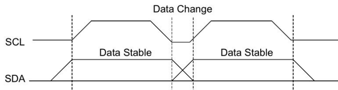
Figure 7.4 Data validity Protocol
