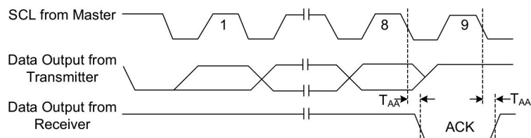
Figure 7.2 Output Acknowledge
