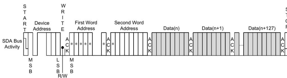
Figure 9.3 Write Security Sector
