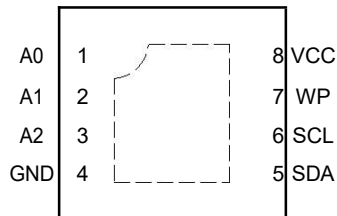
Figure 5.2 8-Lead UDFN
