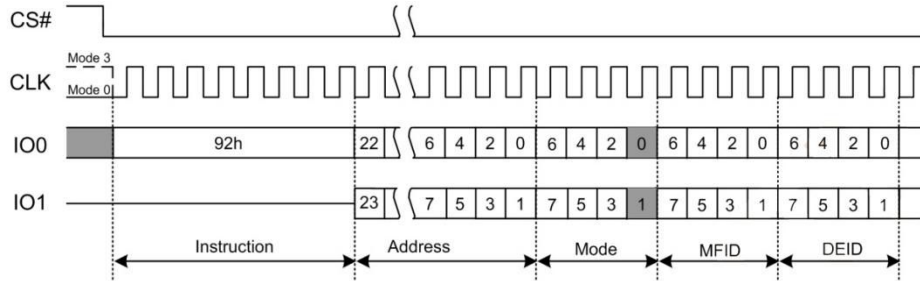
Figure 7.36 Read Manufacturer/Device ID Dual I/O Instruction
