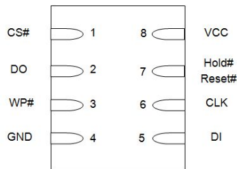
Figure 3.2 8-Contact 6 x 5 mm WSON
