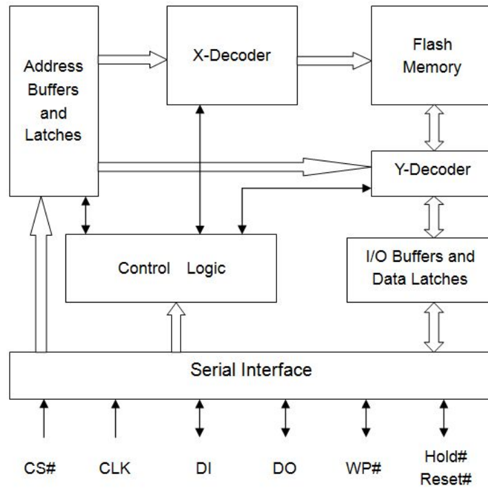
Figure 2.1 Block Diagram
